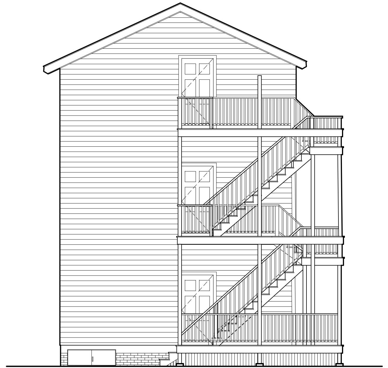
1 Existing Exterior Elevation scale: 3/16" = 1'-0"
