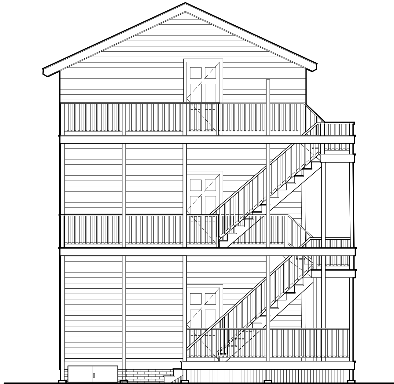
1 Proposed Exterior Elevation scale: 3/16" = 1'-0"
