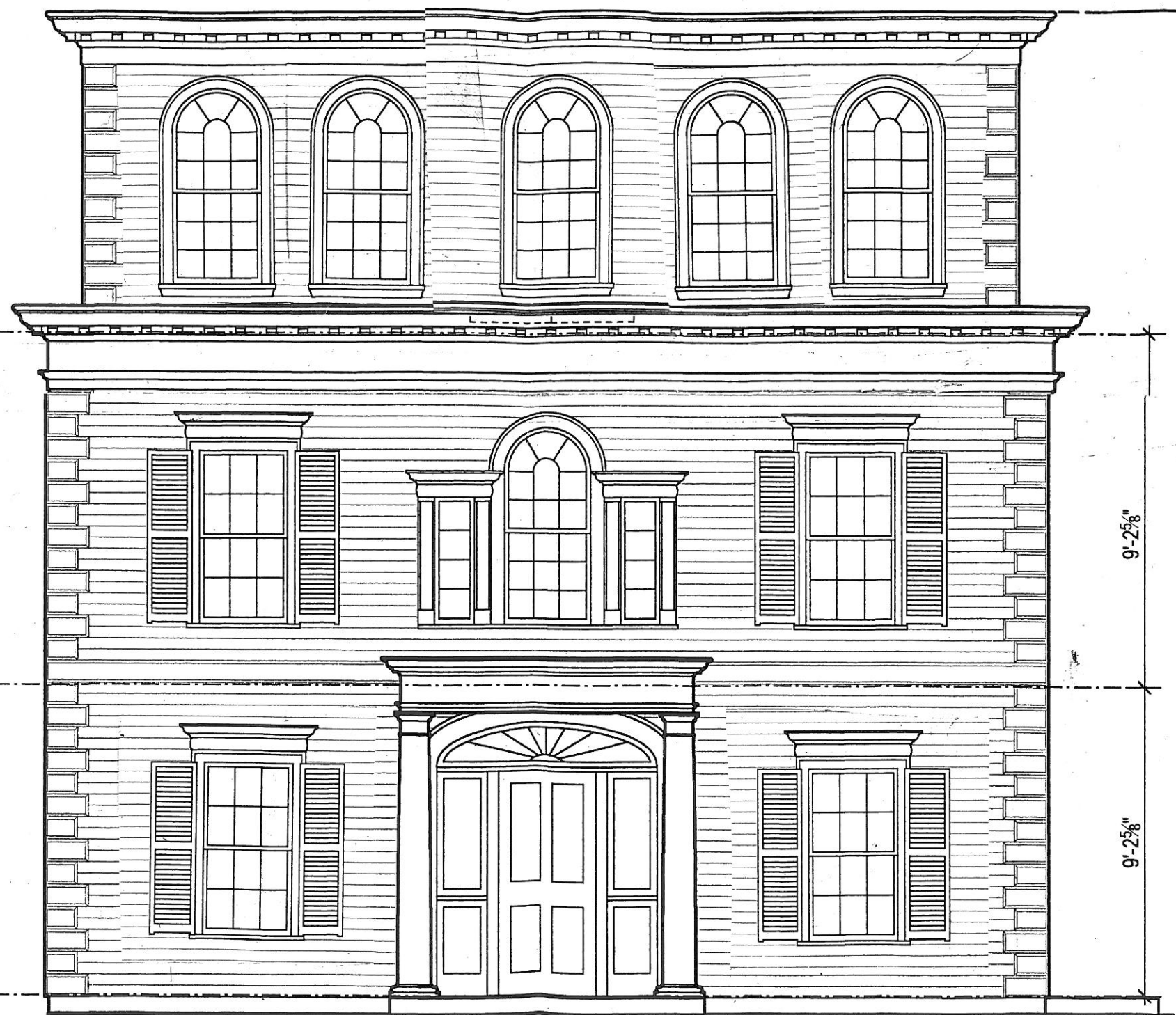
REAR + FRONT ELEVATION
