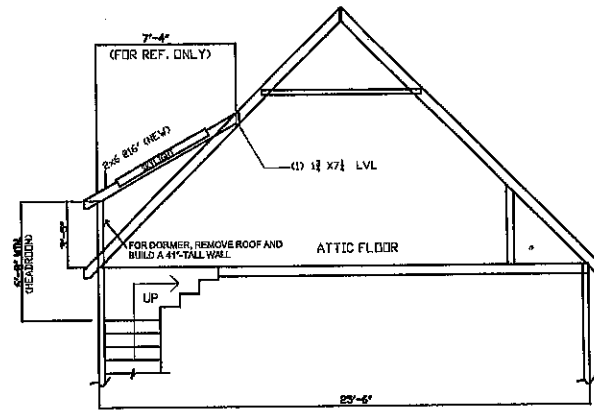
SECTION 1-1 SECTION THRU DORMER
