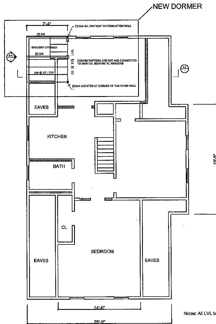
ROOF FRAMING
