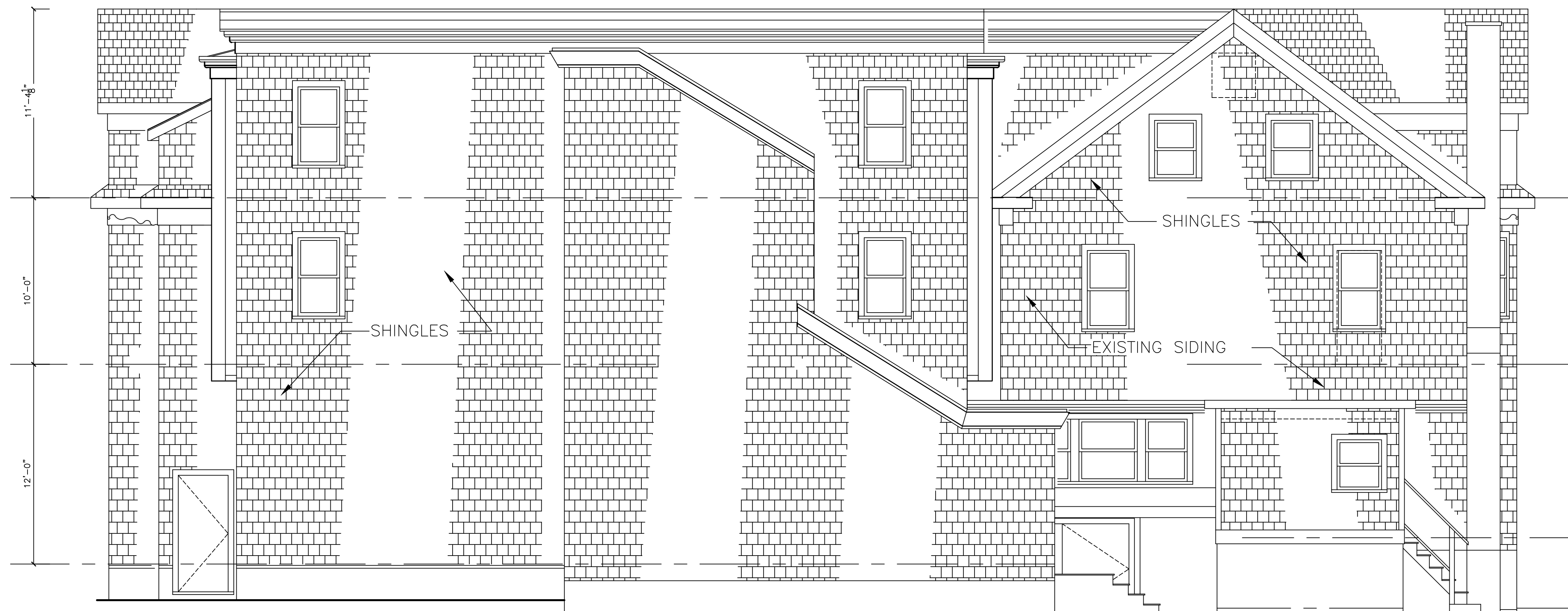
D REAR ELEVATION DD 2 \frac{1}{8}'' = 1' - 0''
