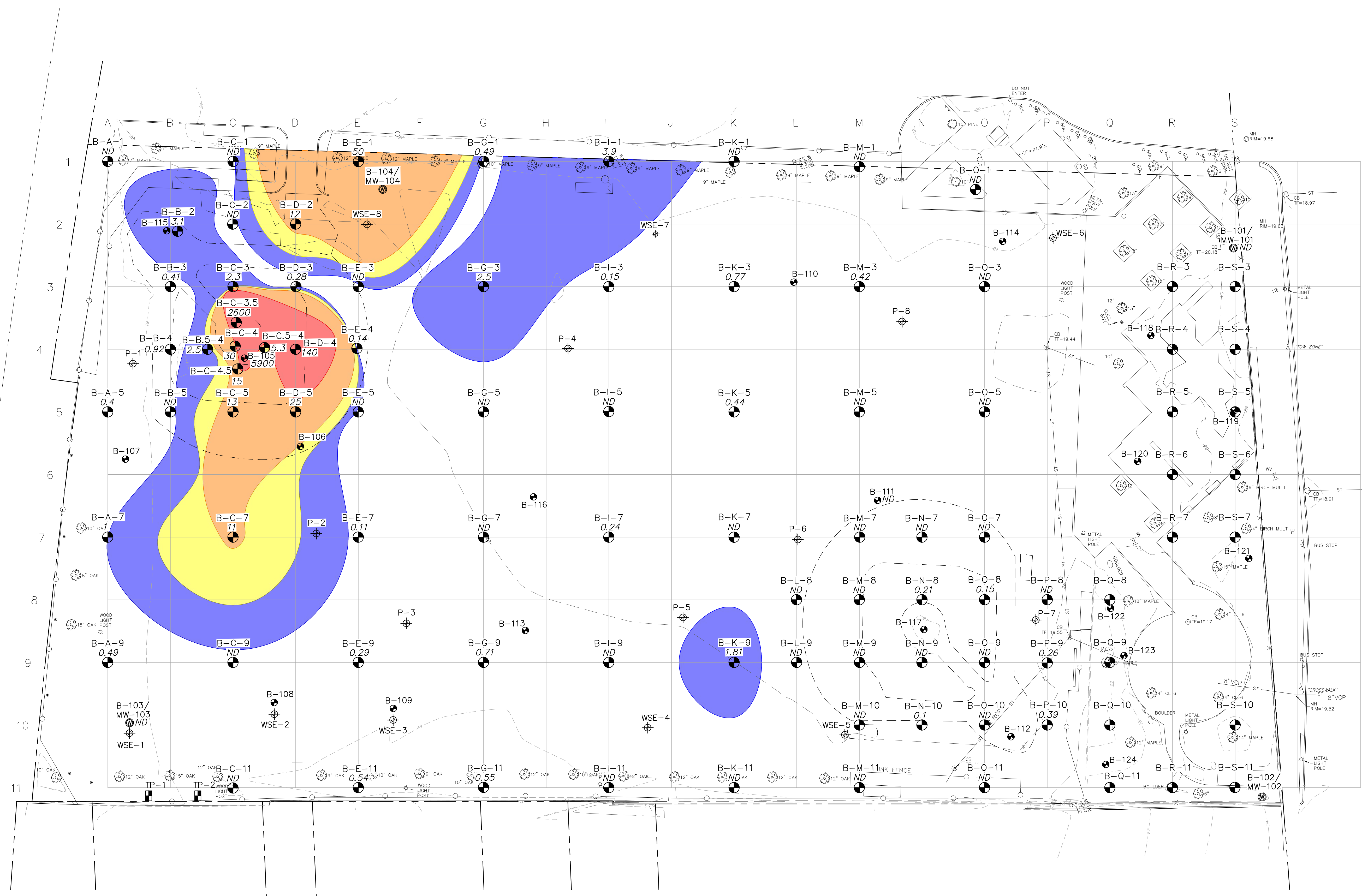
FIGURE 5F CITY OF SOMERVILLE, MASSACHUSETTS CONWAY PARK PCB DISTRIBUTION PLAN: 5.5 - 7.5 FEET JANUARY 2019 SCALE: 1" = 20'
