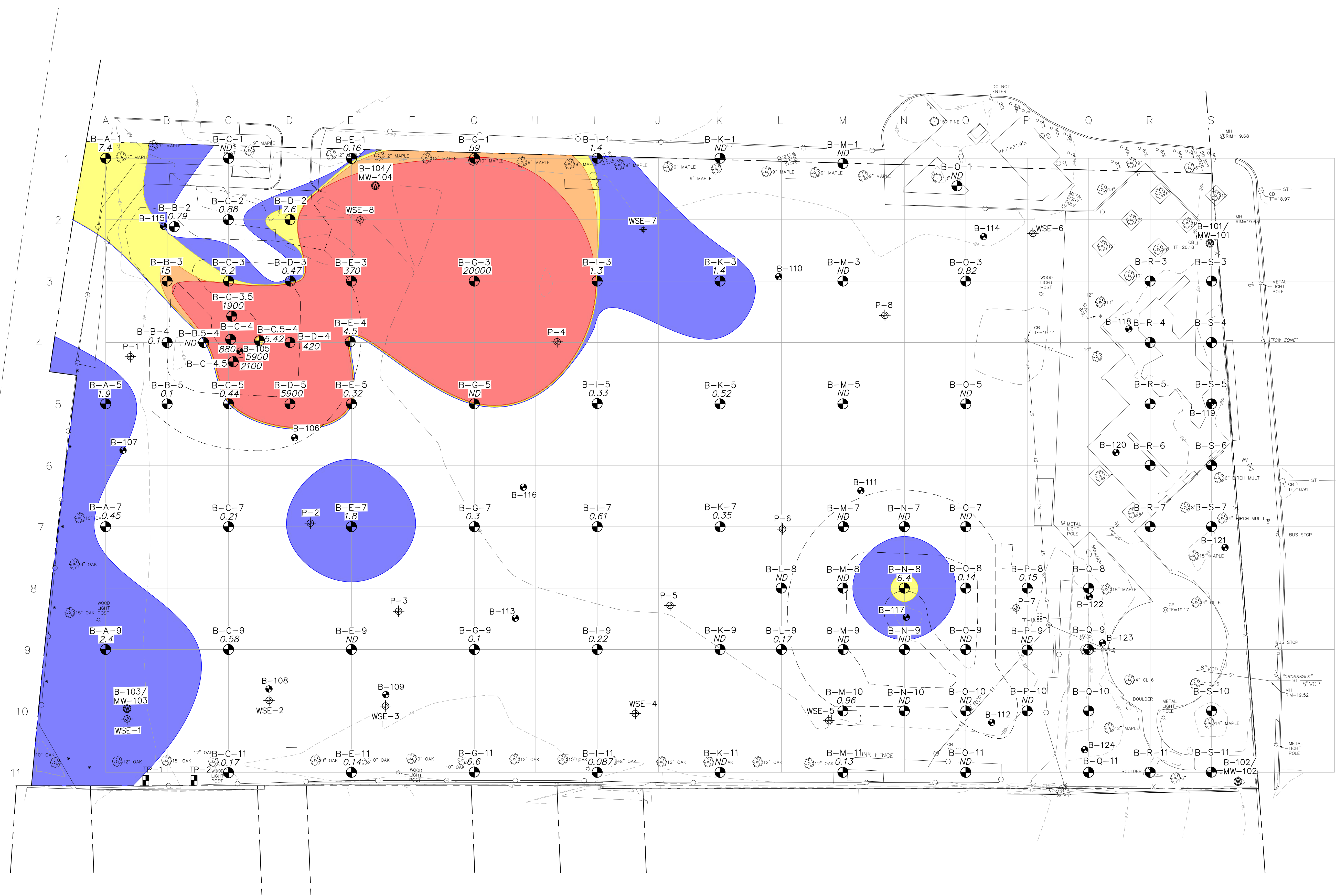
FIGURE 5E CITY OF SOMERVILLE, MASSACHUSETTS CONWAY PARK PCB DISTRIBUTION PLAN: 3.5 - 5.5 FEET JANUARY 2019 SCALE: 1" = 20'
