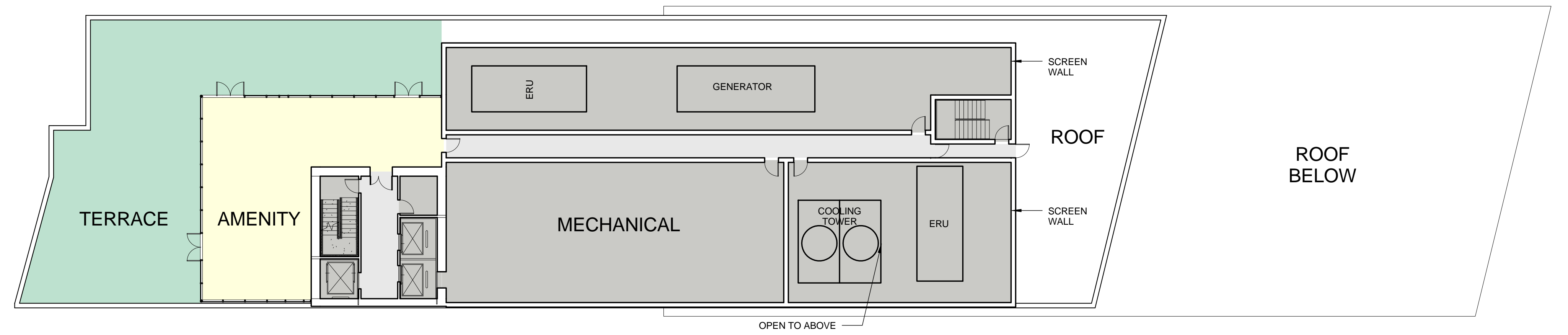
3 ROOF PLAN - LEVEL 20 1/16" = 1'-0"
