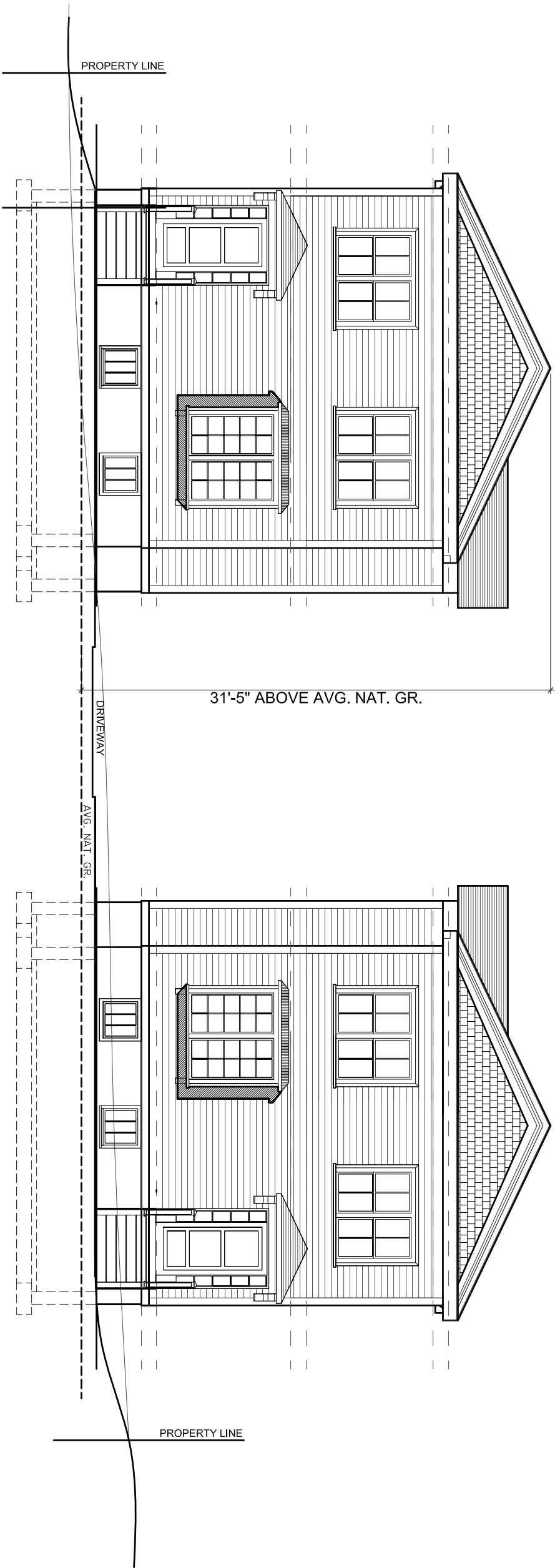
PROPOSED ELEVATION FROM FAIRVIEW TERRACE
